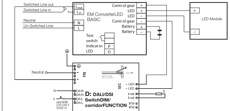
Circuit diagram DE: DALI/DSI/SwitchDIM/corridorFUNCTION + E-kit
